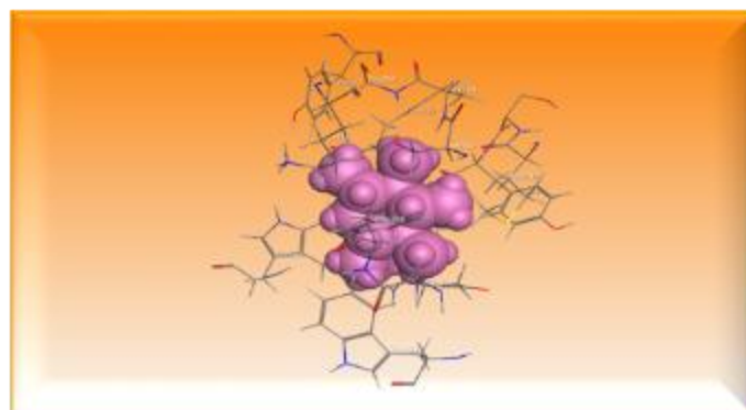
Complexe 5GQB-Ligand de Co-cristallisation. D-Glucosamin.
