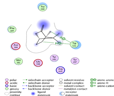
Interaction 5GQB-CAMPBRE
