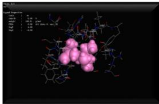
complexe 4ARX-DIMETHOATE
