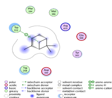
Interaction 5GQB-A-PINENE
